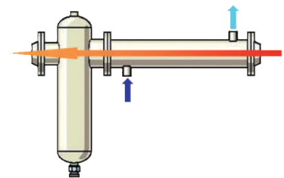
Removable version with ribbed tubes ensures high performance with low pressure drops, designed for easy maintenance
